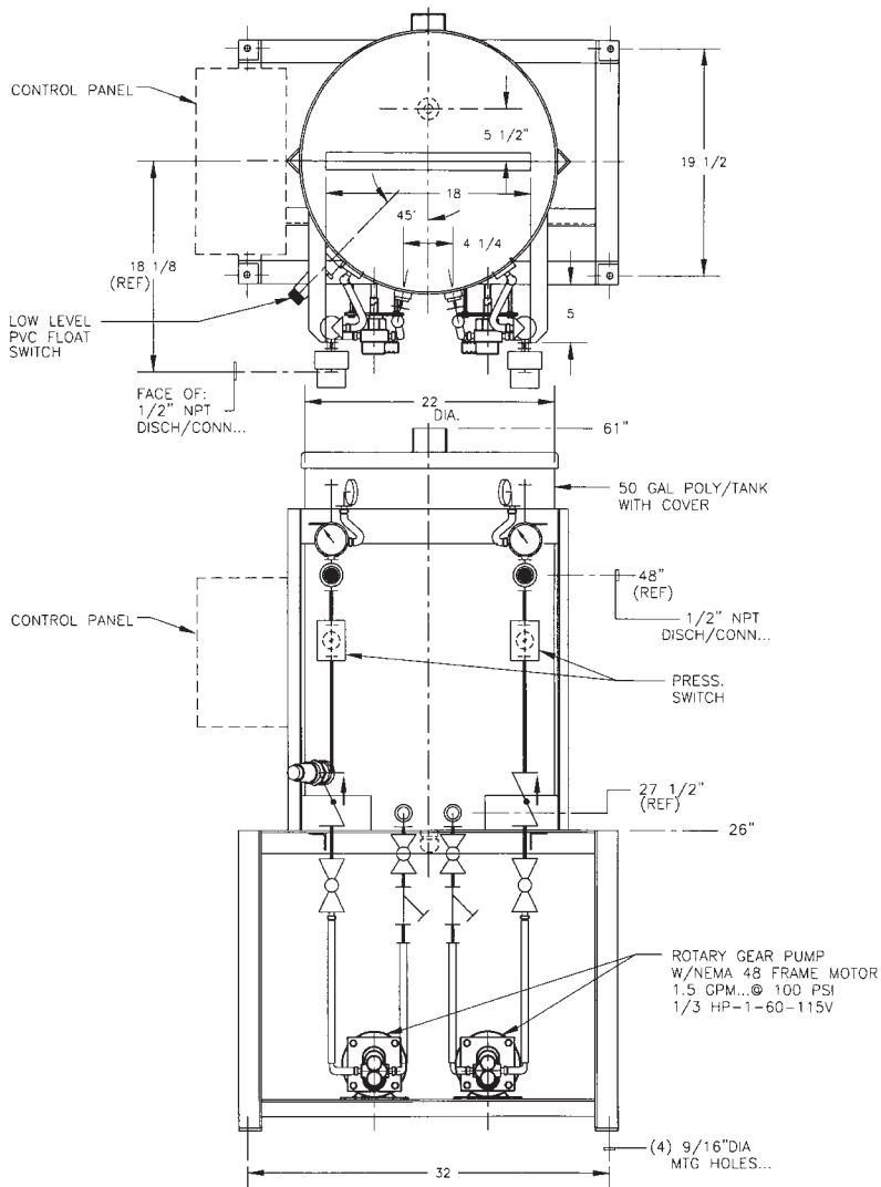
MODEL G-50-2A
